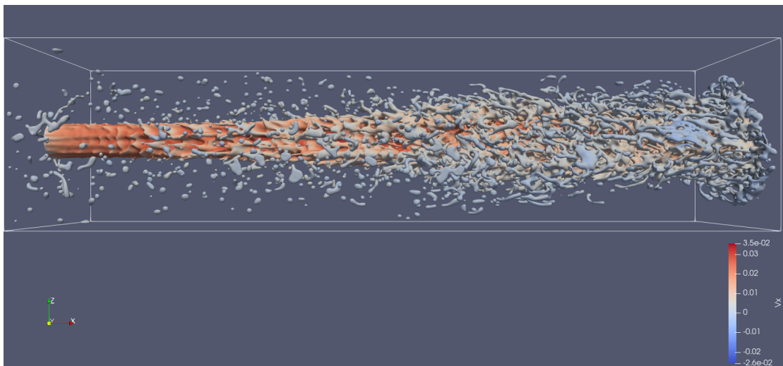
Figure 2: The overall flow structure in a liquid jet breakup with density ratio \frac{\rho_h}{\rho_l} = 1000 , Re = 2000 , We = 133333 .
