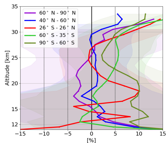
Figure 1: Relative differences between collocated OMPS-LP retrievals and ozonesonde profiles as a function of altitude in several latitude bands, 2012-2020 data.
